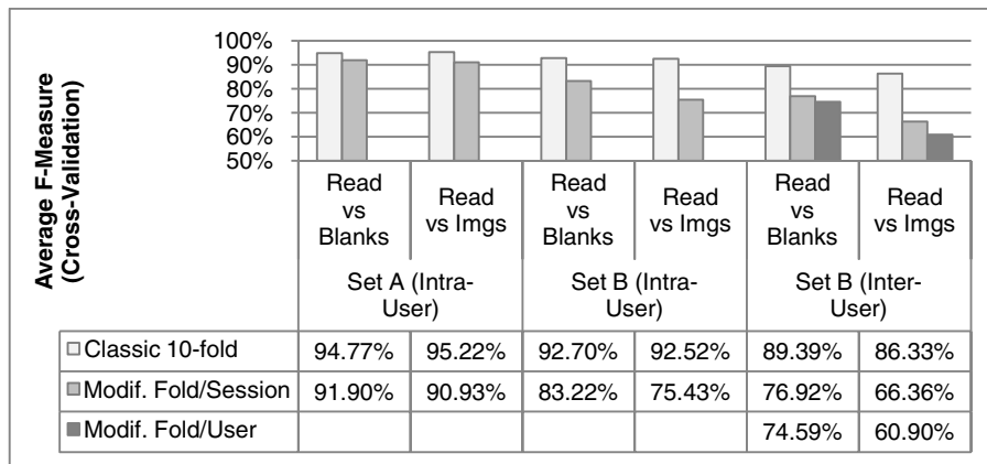
Fig. 4. Silent Reading Detection Results
